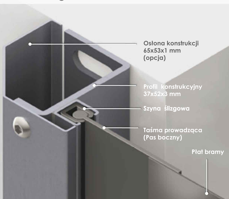
Technologia GRAVITY
